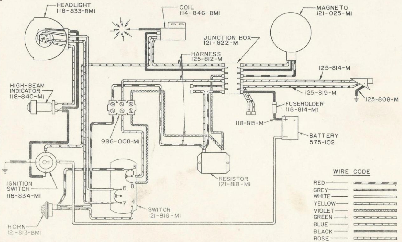
WIRING DIAGRAM
